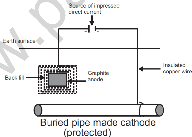
FIGURE: IMPRESSED CATHODIC PROTECTION
